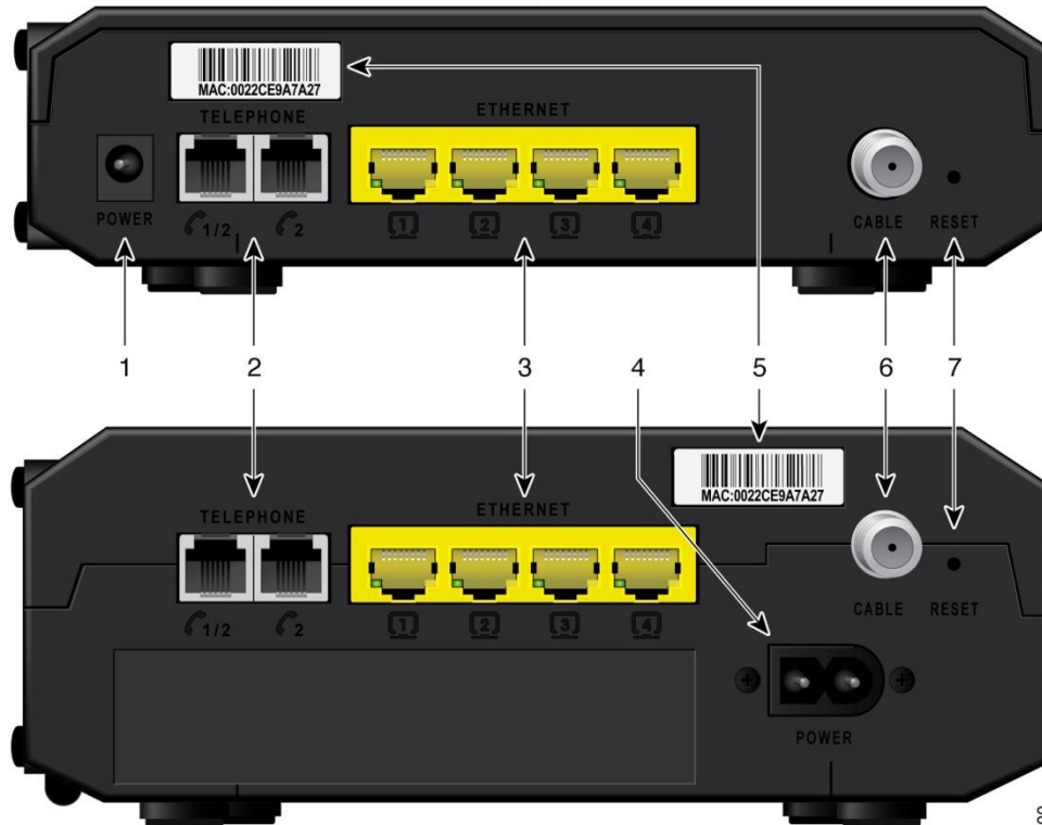
Model DPC2425R2 (Battery Enclosure)
